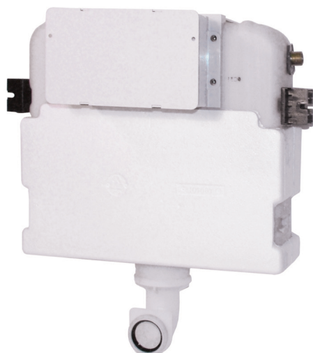
Concealed Dual Flush Cistern - 820mm
